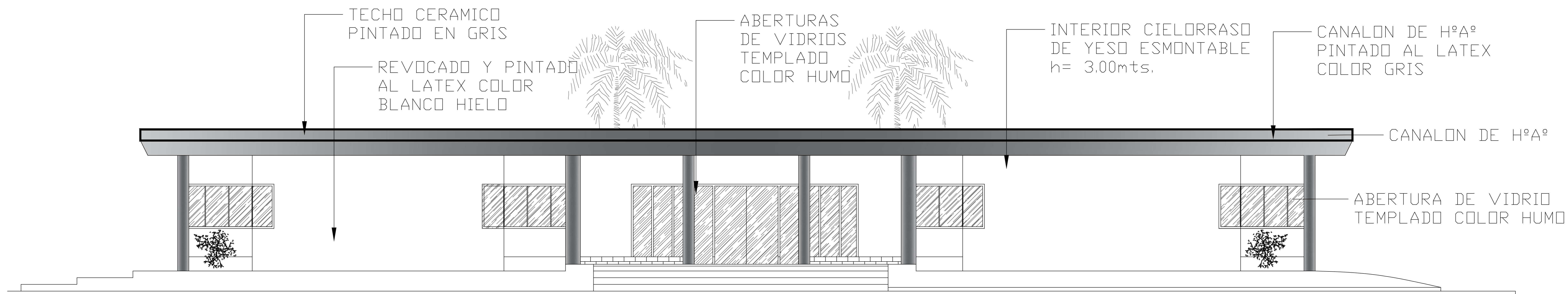
FACHADA PRINCIPAL
