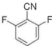
2,6-Difluorobenzonitrile
